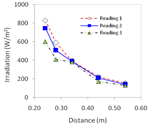
Fig. 5 Irradiation versus distance for one spotlight
