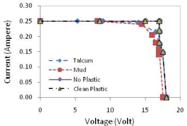
Fig. 7 I-V characteristics for irradiation of 255 W/m 2
