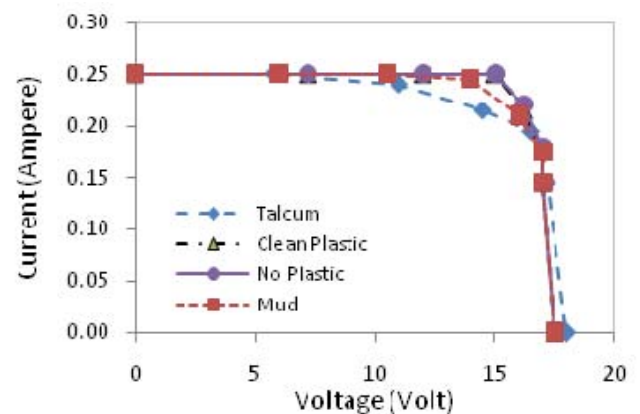
Fig. 8 I-V characteristics for irradiation of 301 W/m 2
